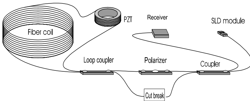
Fig.1 Conventional open loop gyro assembly. S- process completed. Loop coupler and the other coupler are fabricated in sequence. One of the fibers between them is cut («Cut break») to form symmetric output of the assembly. Residual fiber is further used for polarizer fabrication.
