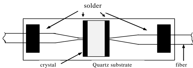
Fig. 2 Fiber crystal polarizer outline.
